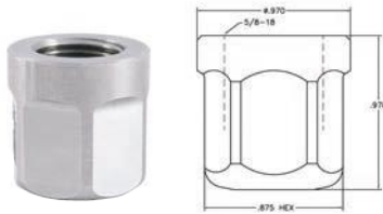
IDNN-HP (Integral Diamond Nozzle Nut) Diamond
